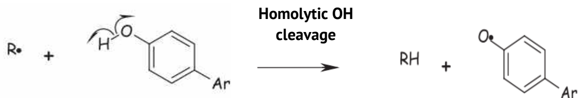
(A) Hydrogen atom transfer (HAT) (1)
