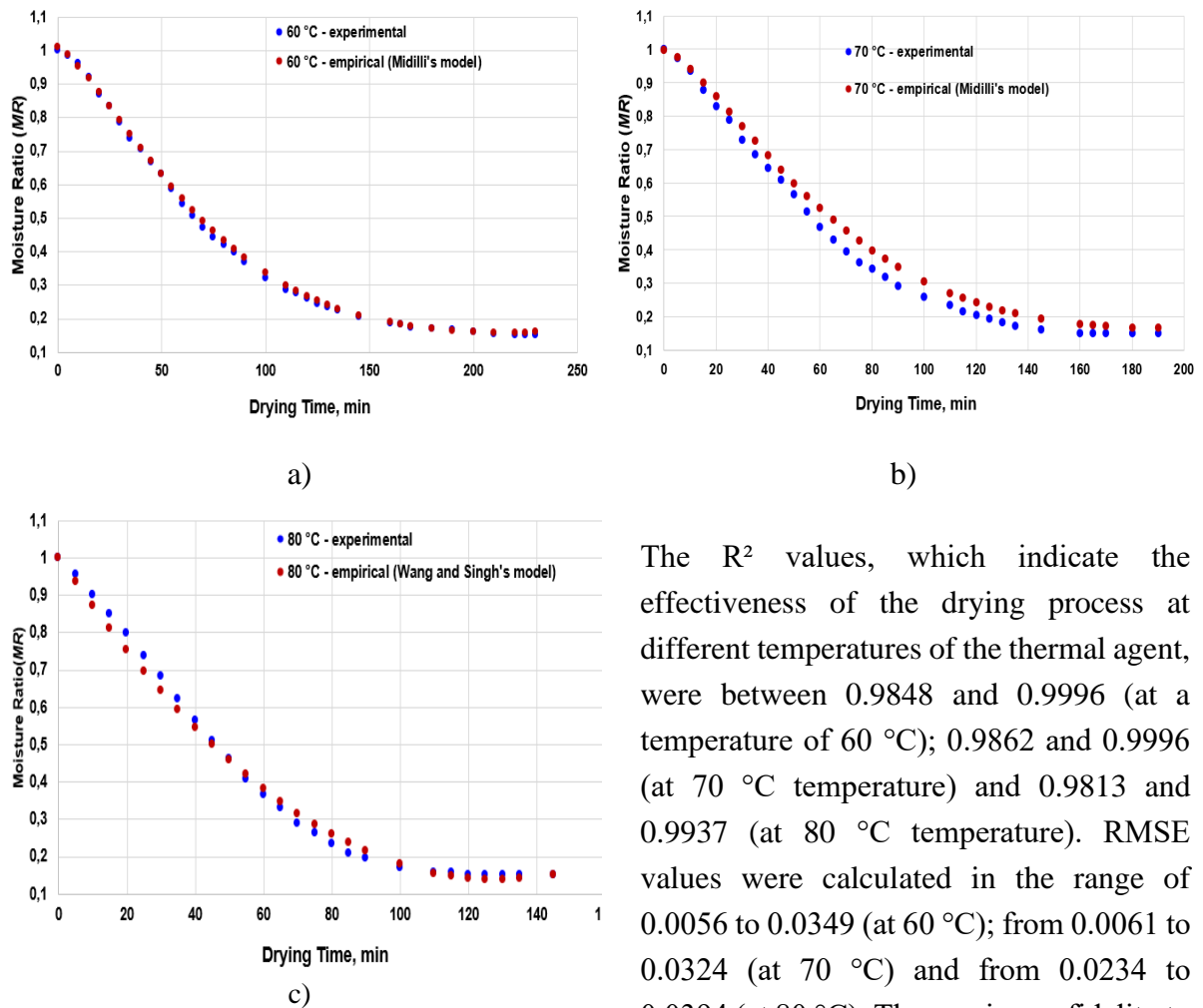
Fig. 3.3. Comparison between experimental and empirical MR according to Midilli's model for the two temperatures studied: a) 60 °C; b) 70 °C and to Wang and Singh's model: c) 80 °C.
